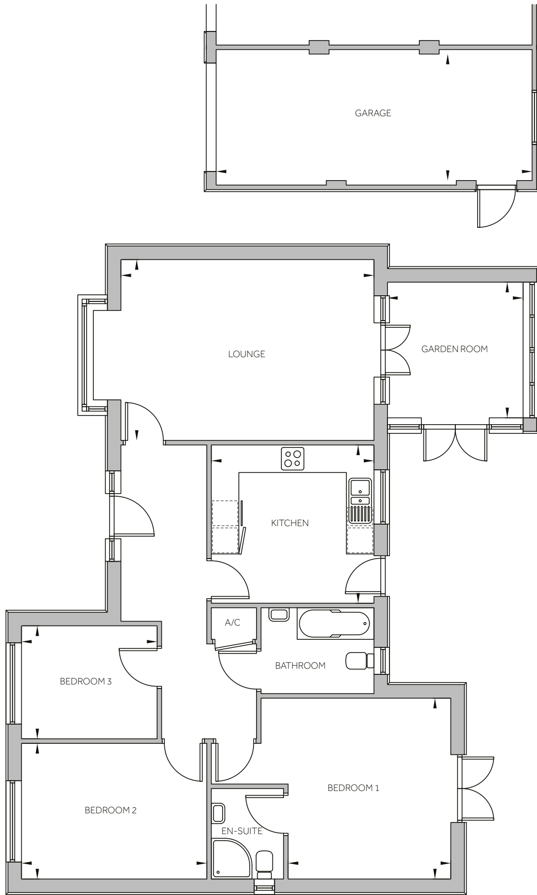
Floor plan indicates Plot 8 Semi detached garage location is indicative only
